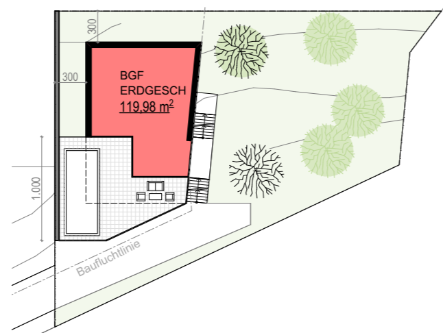
ERDGESCHOSS M1:500
